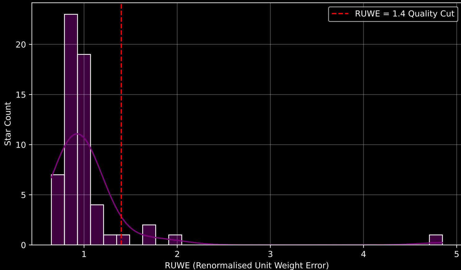
GAPOGEE DR17 Field [279-35-O] RUWE Distribution (n= 59)
