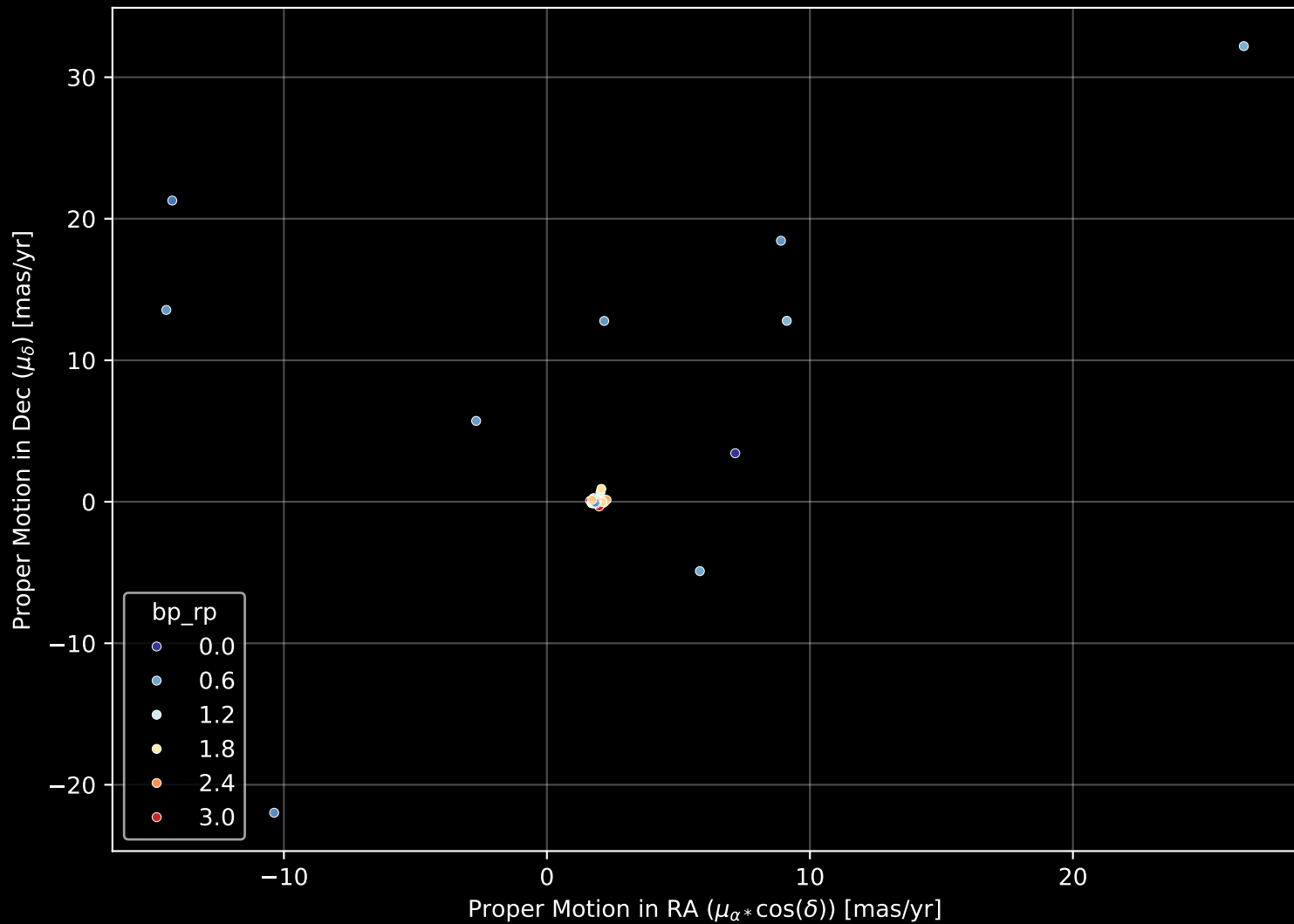
APOGEE DR17 Field: [279-35-O] Proper Motion Diagram (n= 59)
