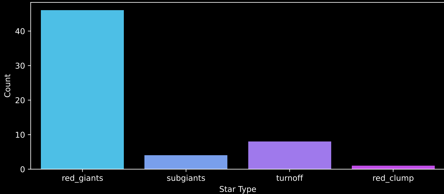
APOGEE DR17 Field: [279-35-O] Count plot of Star Type
