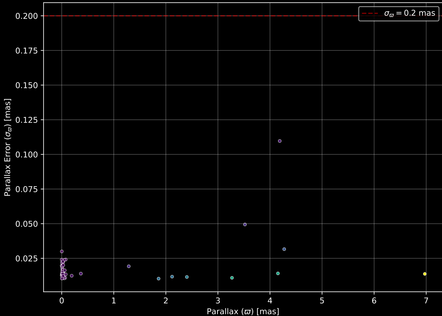
APOGEE DR17 Field: [279-35-O] Parallax Quality (n= 59)
